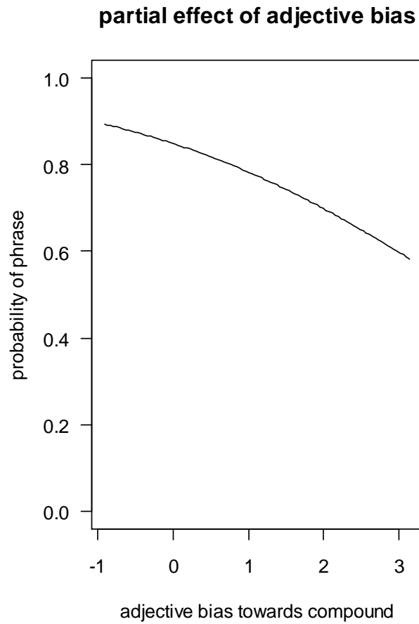
Figure 4: Effect of adjective bias on choice of construct, gradient family bias, data set with only neutral constituents (N=530). Larger values on the x-axes mean a greater bias for the compound.
